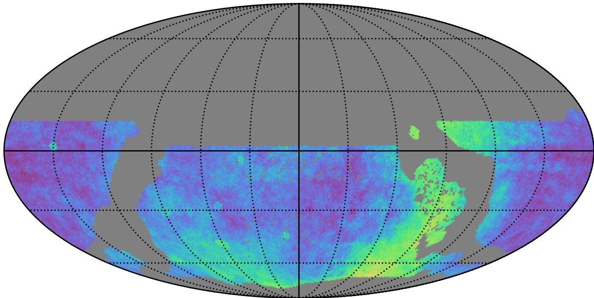
too_elab_r8_d3_gz_v3.4_10yrs WFD: Parallax Coverage @ 22.4
