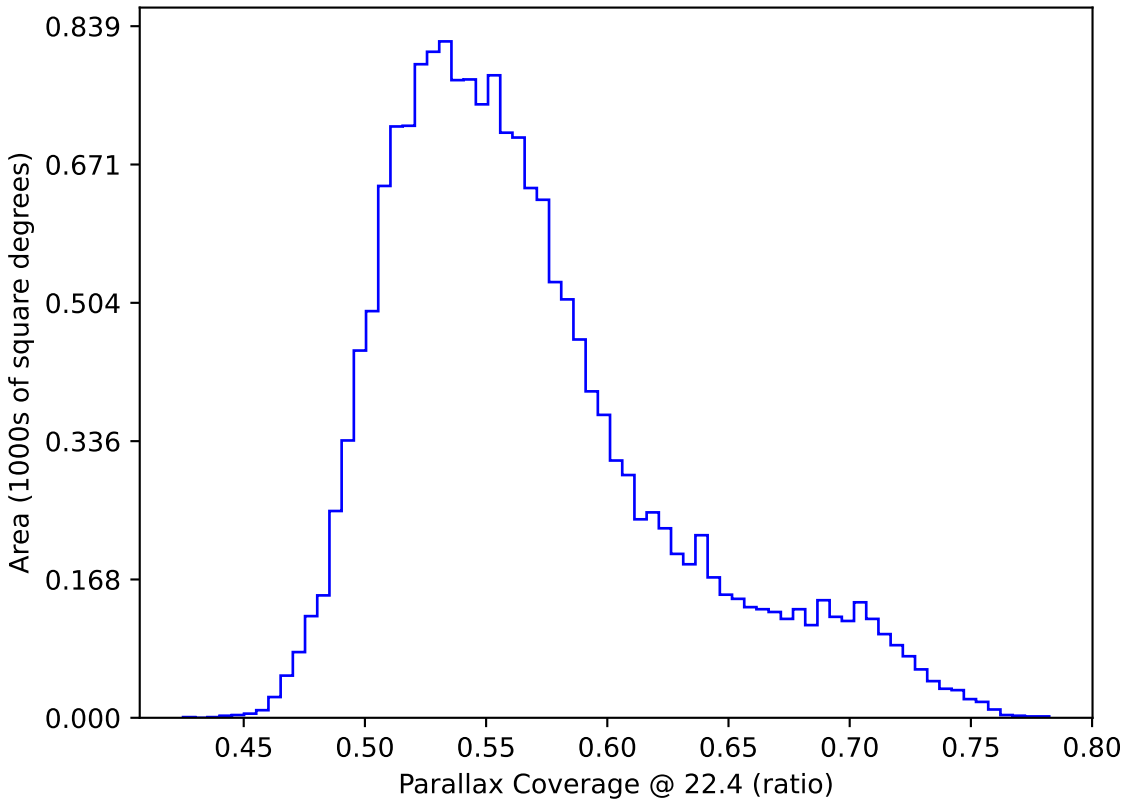
too_elab_r8_d3_gz_v3.4_10yrs WFD: Parallax Coverage @ 22.4
