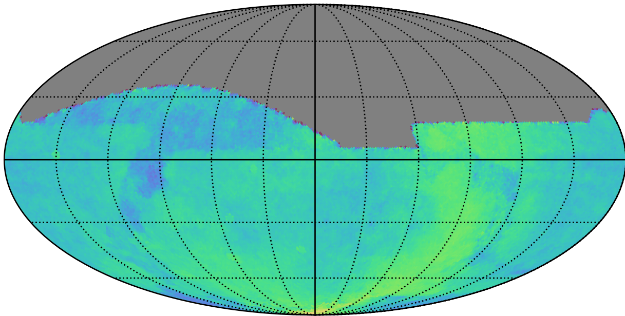
too_elab_r8_d3_gz_v3.4_10yrs All sky: Parallax Coverage @ 22.4
