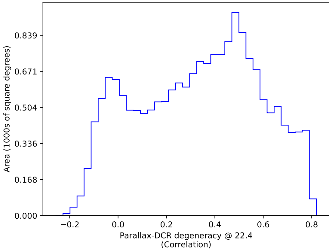
too_elab_r8_d3_gz_v3.4_10yrs WFD: Parallax-DCR degeneracy @ 22.4
