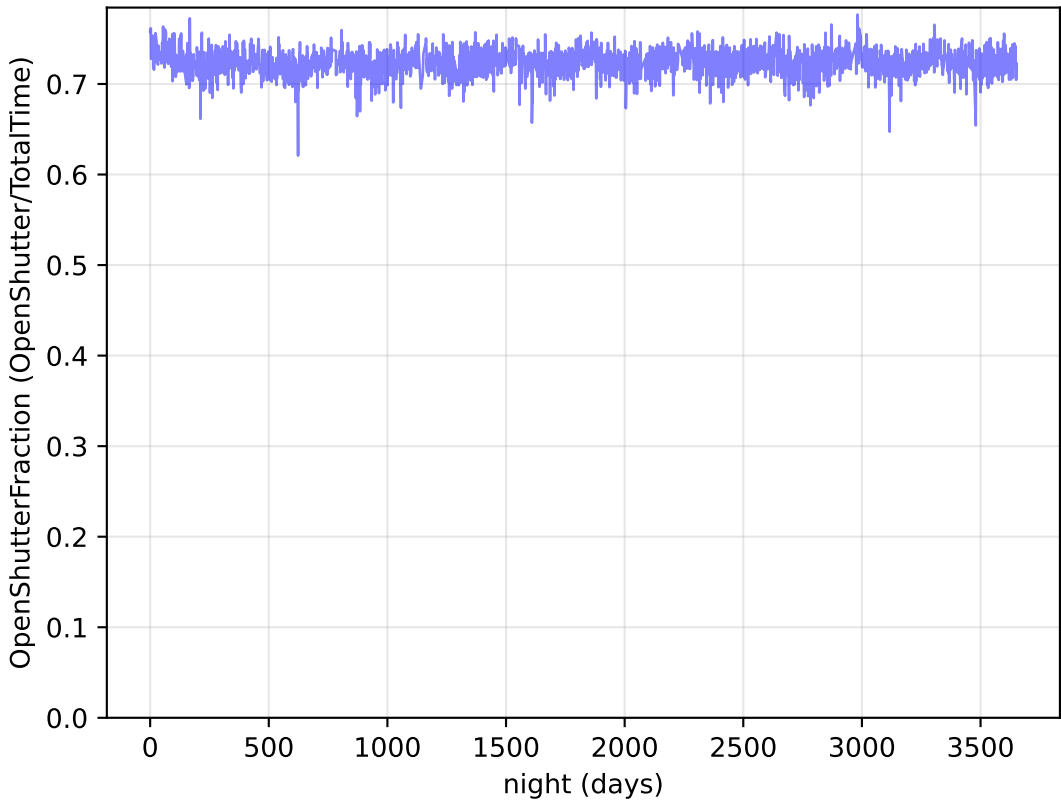
too_elab_r8_d3_gz_v3.4_10yrs Per night: OpenShutterFraction
