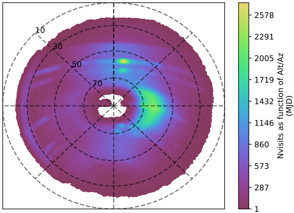
too_elab_r8_d3_gz_v3.4_10yrs r band: Nvisits as function of Alt/Az
