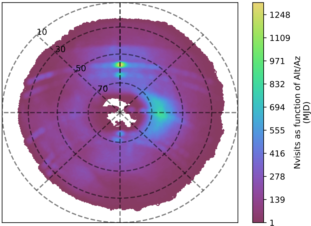
too_elab_r8_d3_gz_v3.4_10yrs g band: Nvisits as function of Alt/Az
