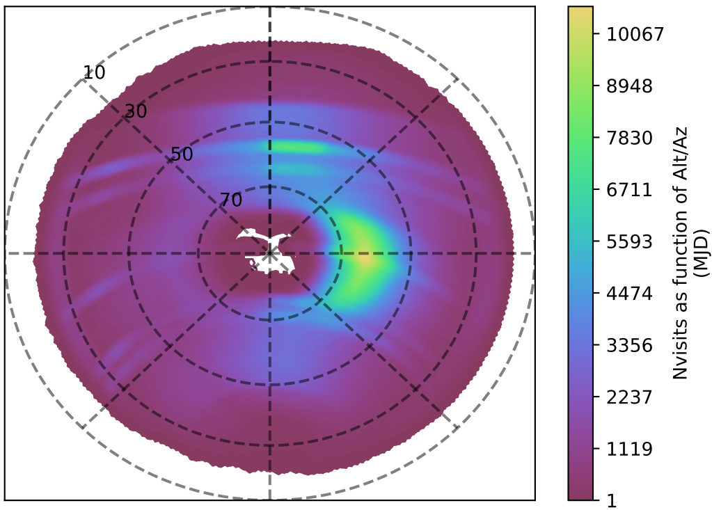
too_elab_r8_d3_gz_v3.4_10yrs all bands: Nvisits as function of Alt/Az
