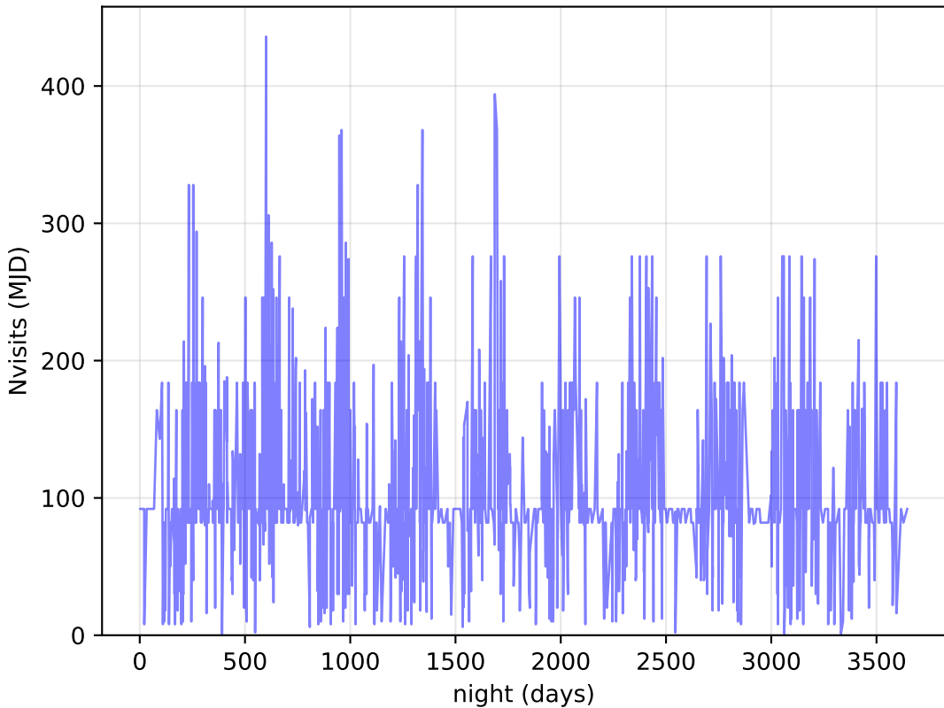
too_elab_r8_d3_gz_v3.4_10yrs DDF: Nvisits
