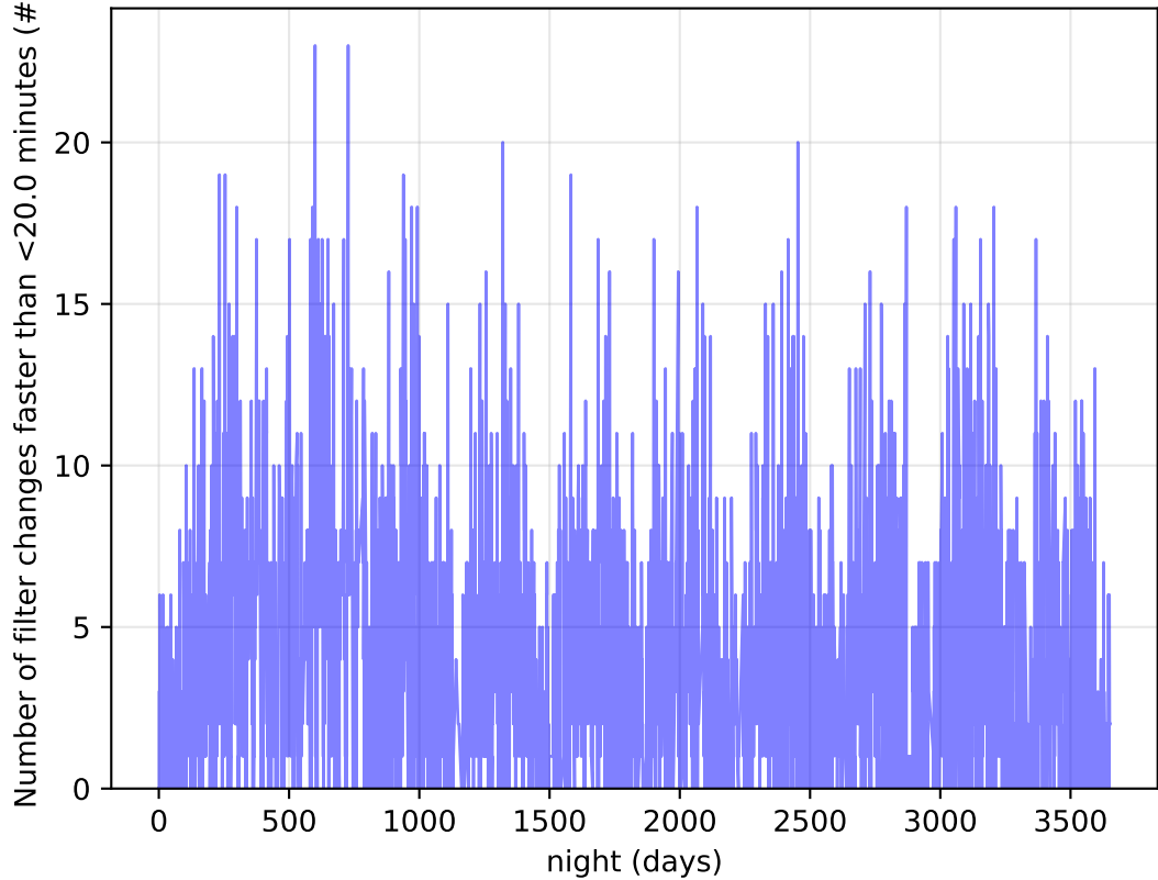
too_elab_r8_d3_gz_v3.4_10yrs Per Night: Number of filter changes faster than <20.0 minutes
