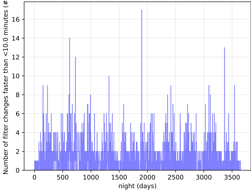
too_elab_r8_d3_gz_v3.4_10yrs Per Night: Number of filter changes faster than <10.0 minutes
