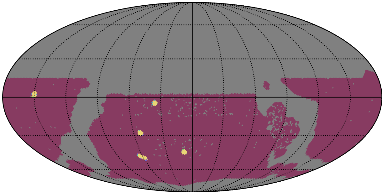
too_elab_r8_d3_gz_v3.4_10yrs WFD: NumberOfQuickRevisits
