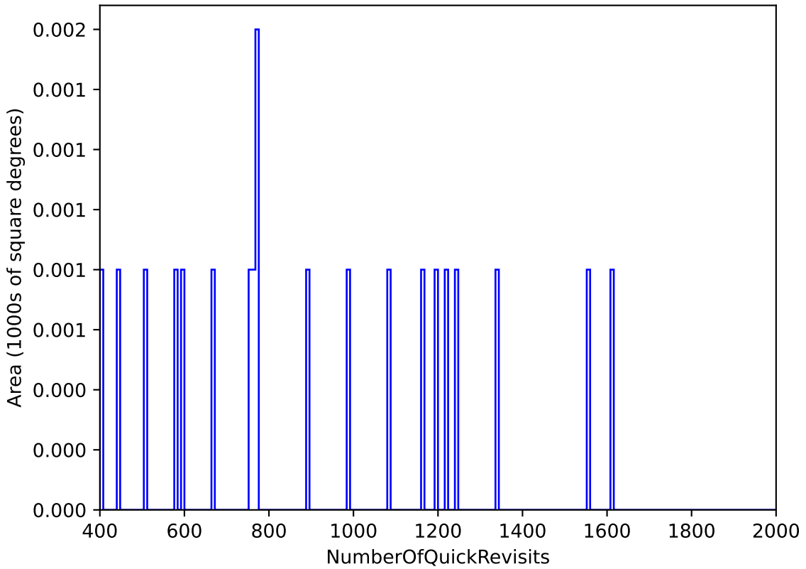
too_elab_r8_d3_gz_v3.4_10yrs WFD: NumberOfQuickRevisits
