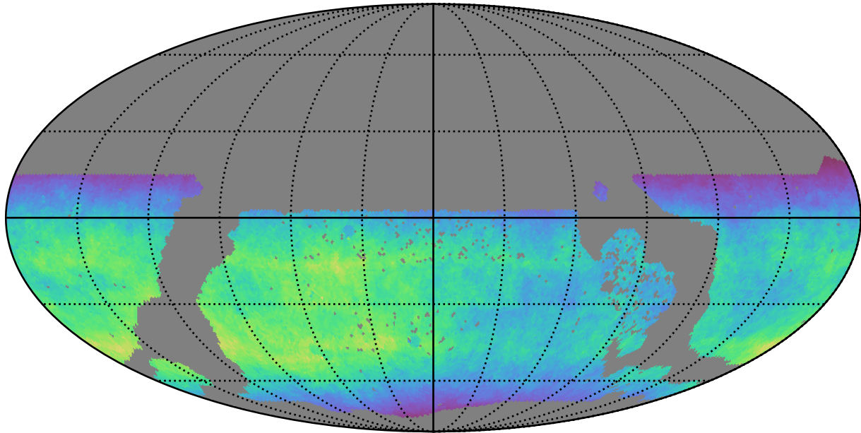
too_elab_r8_d3_gz_v3.4_10yrs WFD y band: Normalized Teff
