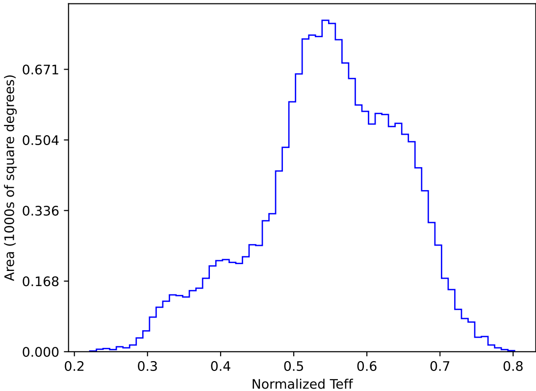
too_elab_r8_d3_gz_v3.4_10yrs WFD y band: Normalized Teff
