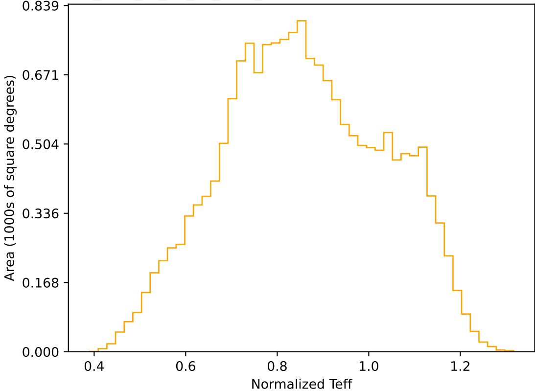
too_elab_r8_d3_gz_v3.4_10yrs WFD r band: Normalized Teff
