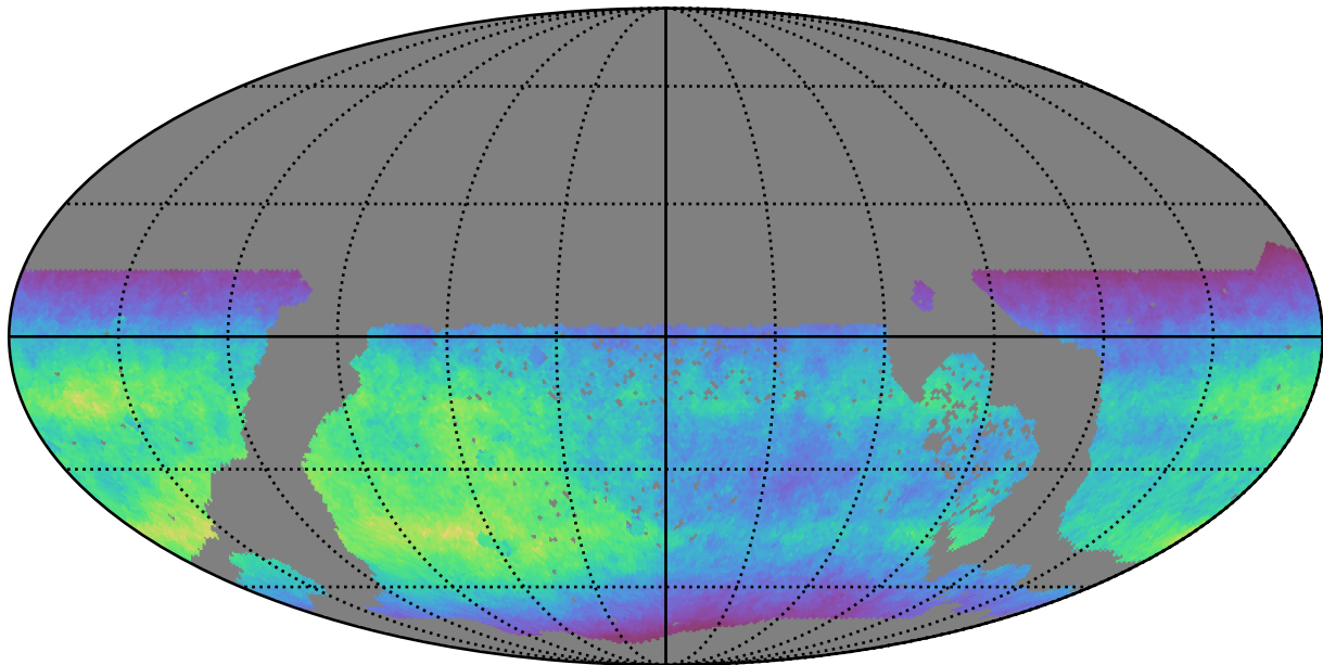
too_elab_r8_d3_gz_v3.4_10yrs WFD i band: Normalized Teff
