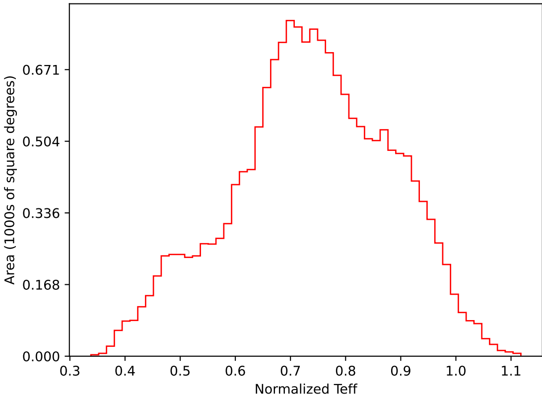
too_elab_r8_d3_gz_v3.4_10yrs WFD i band: Normalized Teff
