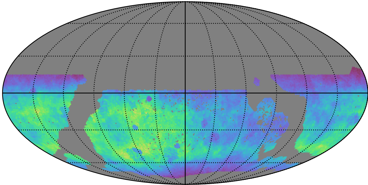
too_elab_r8_d3_gz_v3.4_10yrs WFD g band: Normalized Teff
