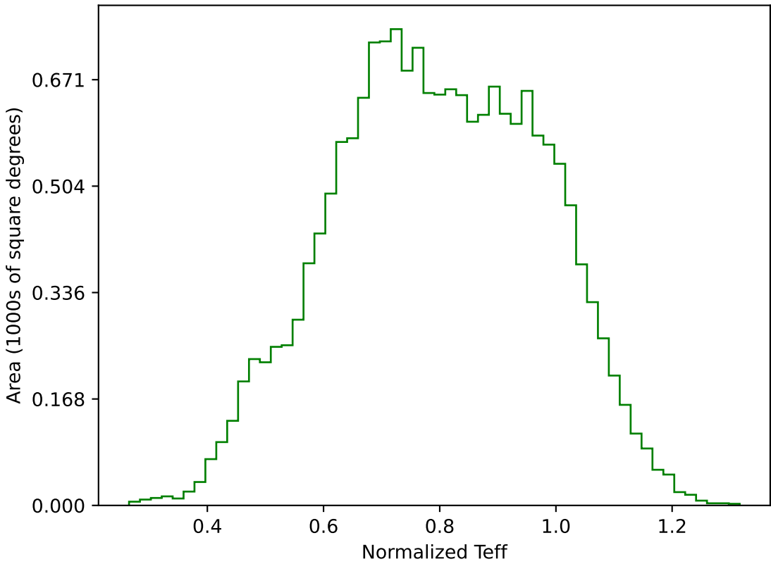
too_elab_r8_d3_gz_v3.4_10yrs WFD g band: Normalized Teff
