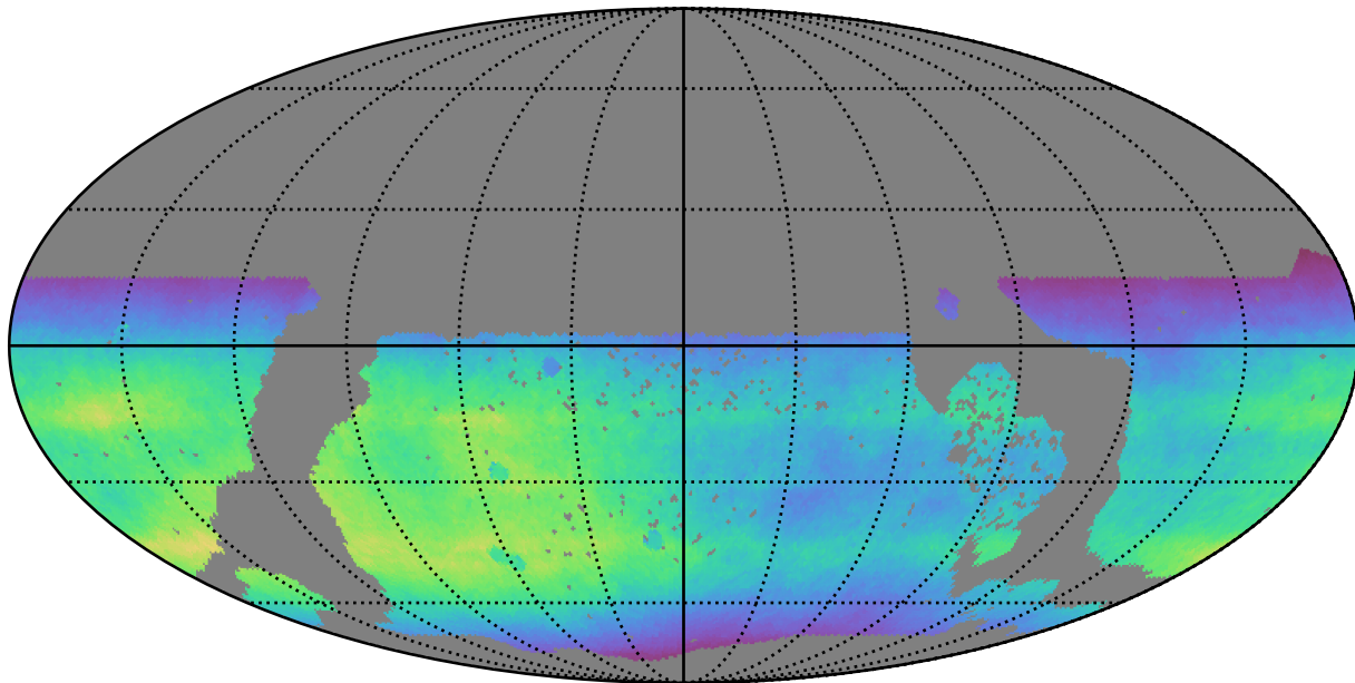
too_elab_r8_d3_gz_v3.4_10yrs WFD all bands: Normalized Teff
