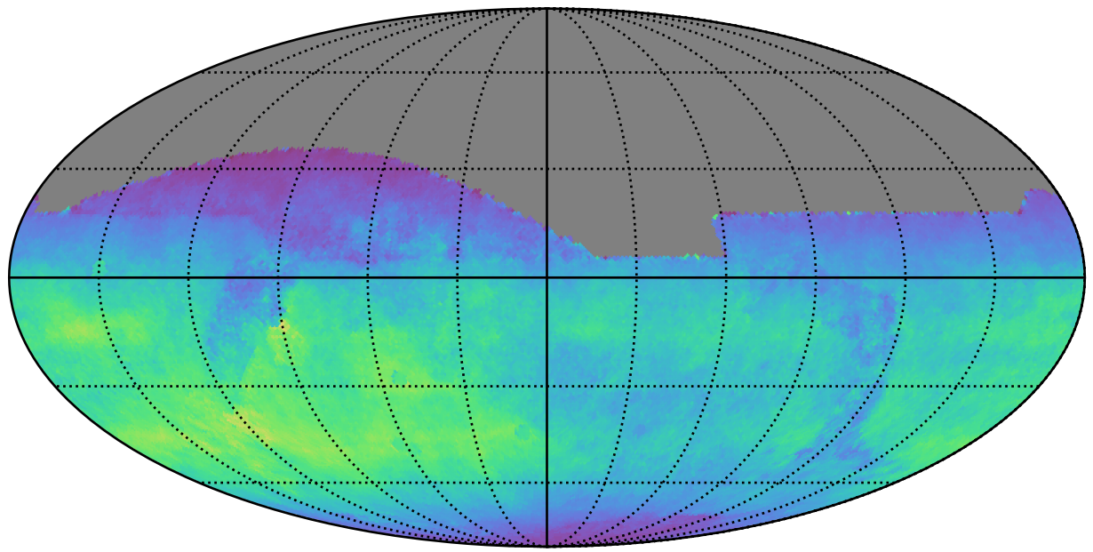
too_elab_r8_d3_gz_v3.4_10yrs All sky z band: Normalized Teff
