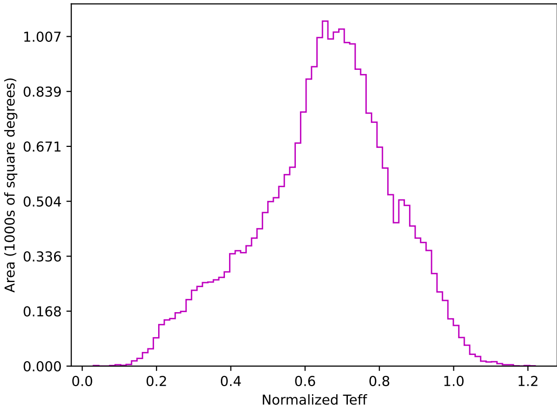
too_elab_r8_d3_gz_v3.4_10yrs All sky z band: Normalized Teff
