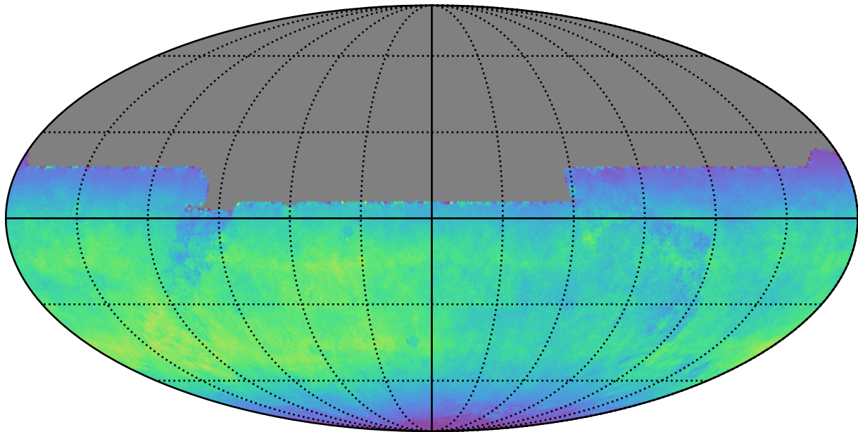
too_elab_r8_d3_gz_v3.4_10yrs All sky y band: Normalized Teff
