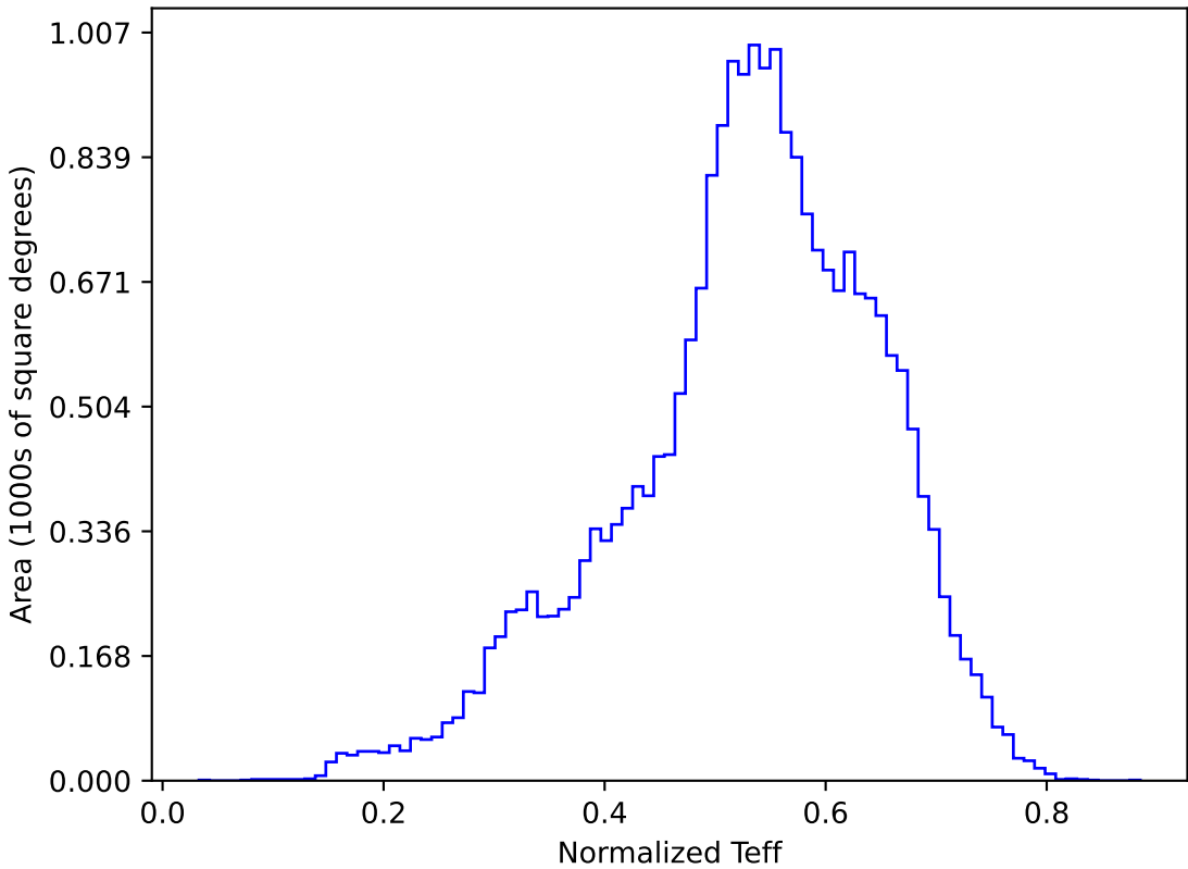
too_elab_r8_d3_gz_v3.4_10yrs All sky y band: Normalized Teff
