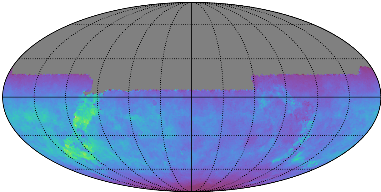
too_elab_r8_d3_gz_v3.4_10yrs All sky u band: Normalized Teff
