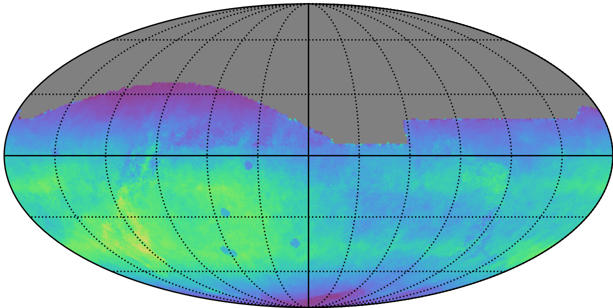
too_elab_r8_d3_gz_v3.4_10yrs All sky r band: Normalized Teff
