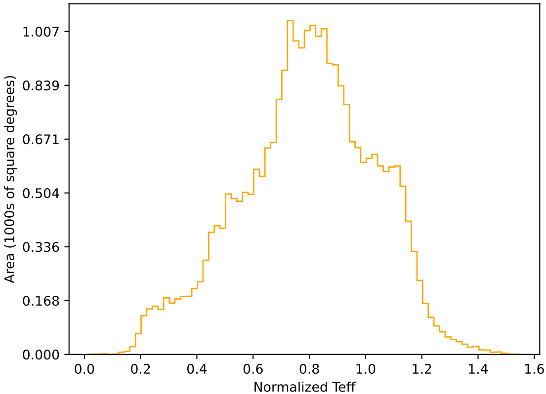
too_elab_r8_d3_gz_v3.4_10yrs All sky r band: Normalized Teff
