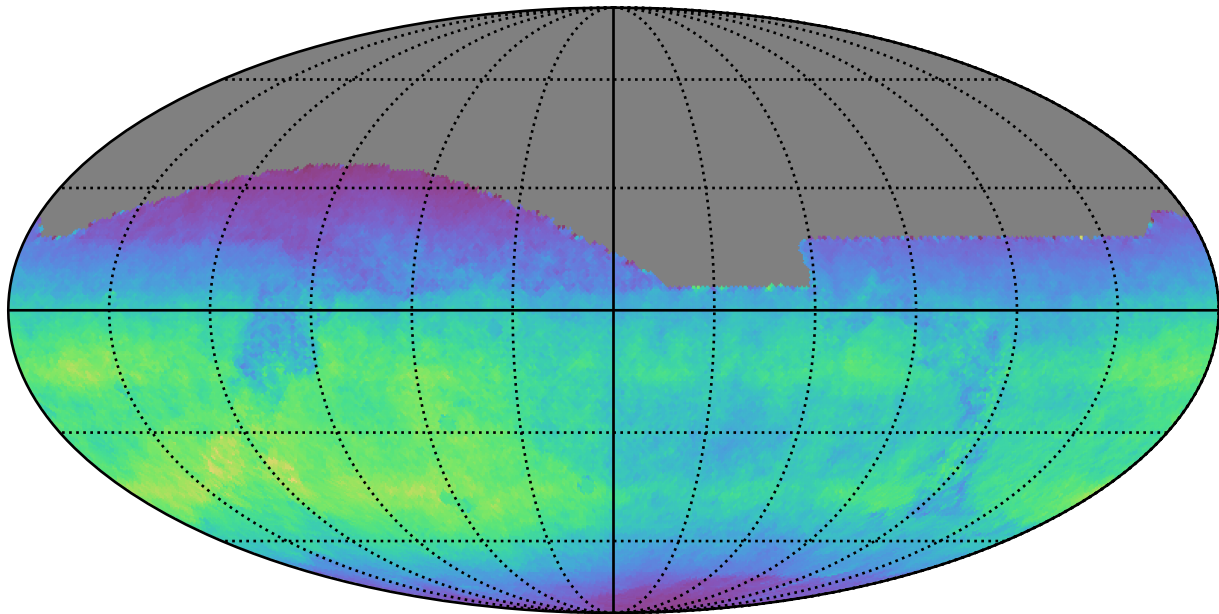
too_elab_r8_d3_gz_v3.4_10yrs All sky i band: Normalized Teff
