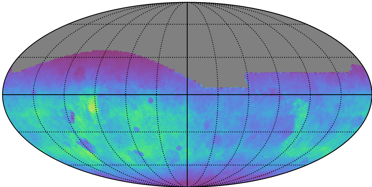
too_elab_r8_d3_gz_v3.4_10yrs All sky g band: Normalized Teff
