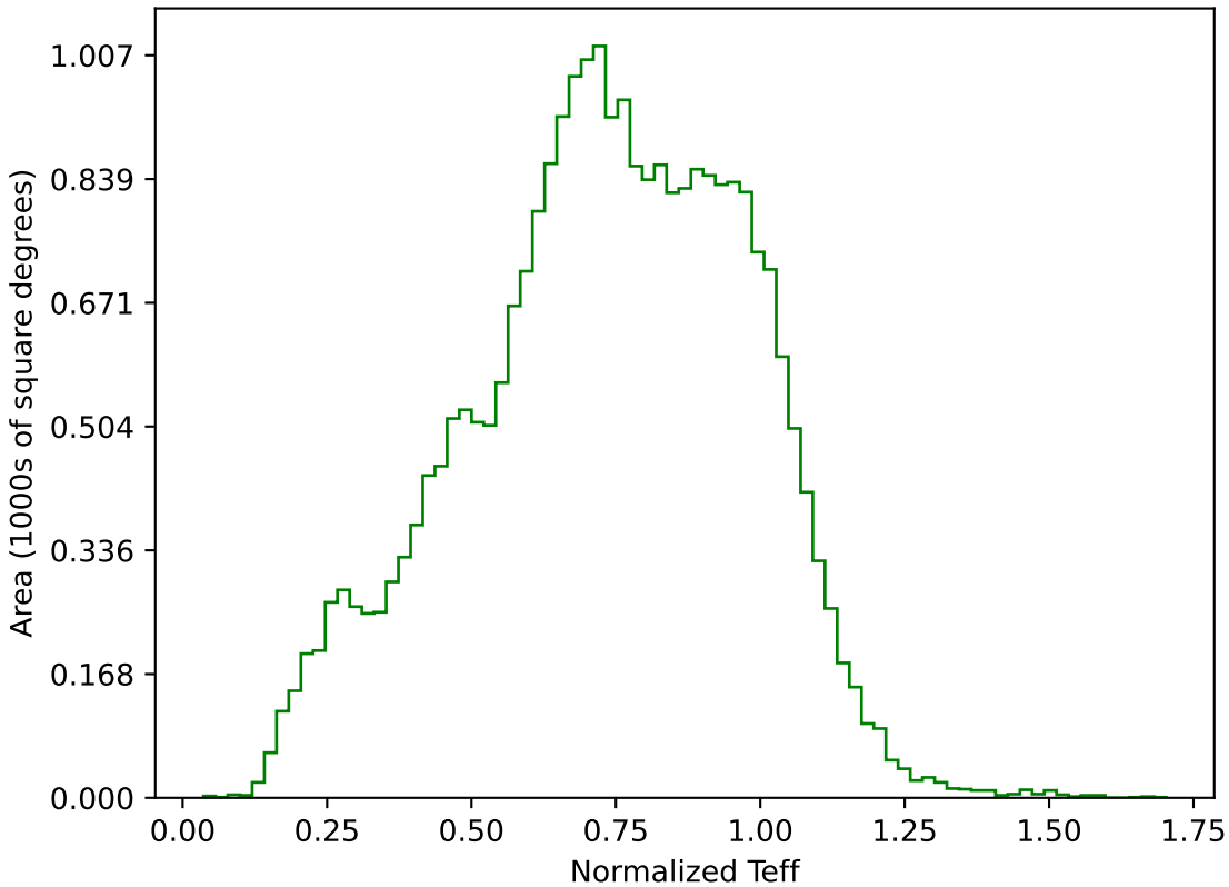
too_elab_r8_d3_gz_v3.4_10yrs All sky g band: Normalized Teff
