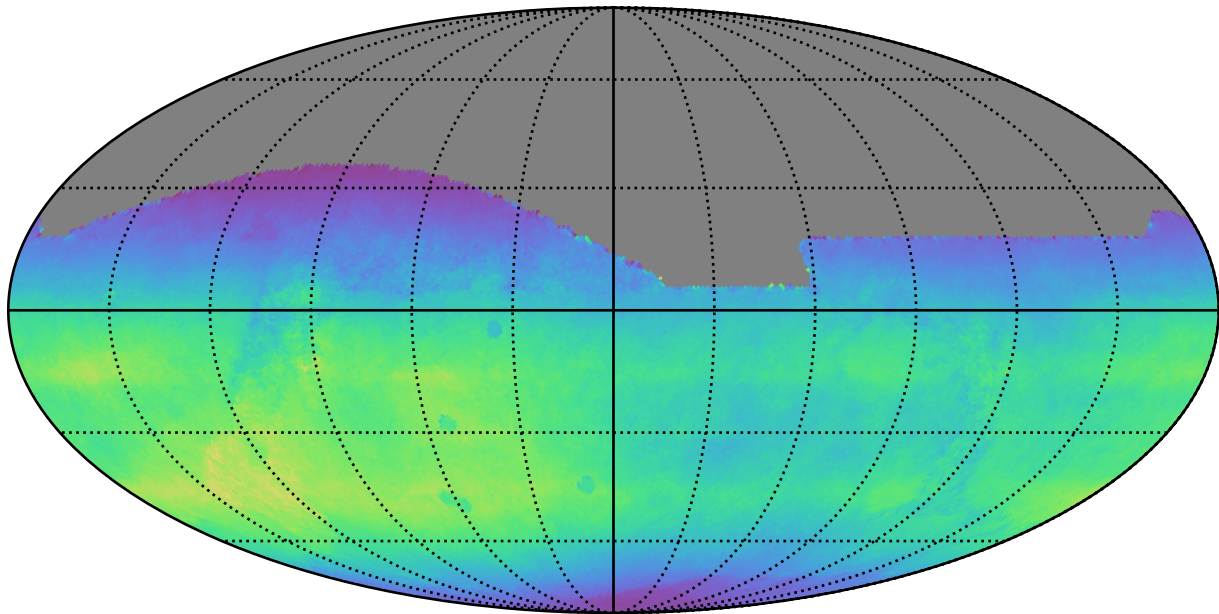
too_elab_r8_d3_gz_v3.4_10yrs All sky all bands: Normalized Teff
