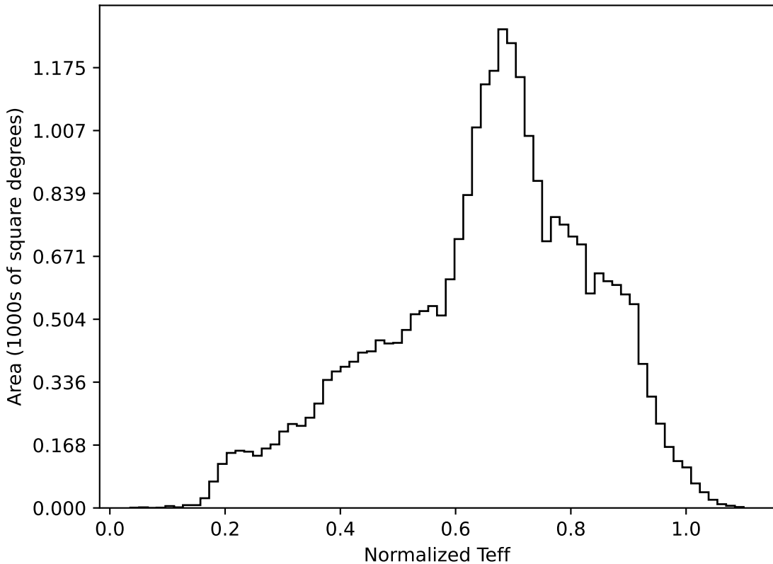
too_elab_r8_d3_gz_v3.4_10yrs All sky all bands: Normalized Teff
