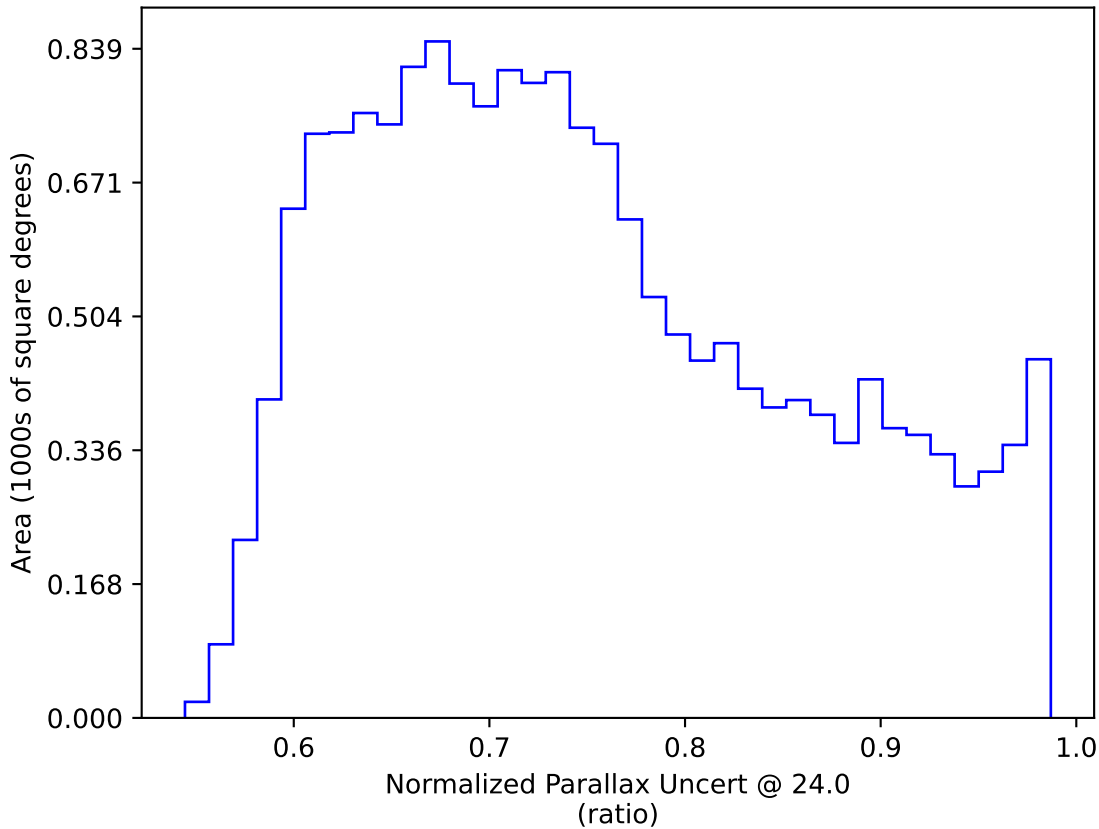
too_elab_r8_d3_gz_v3.4_10yrs WFD: Normalized Parallax Uncert @ 24.0
