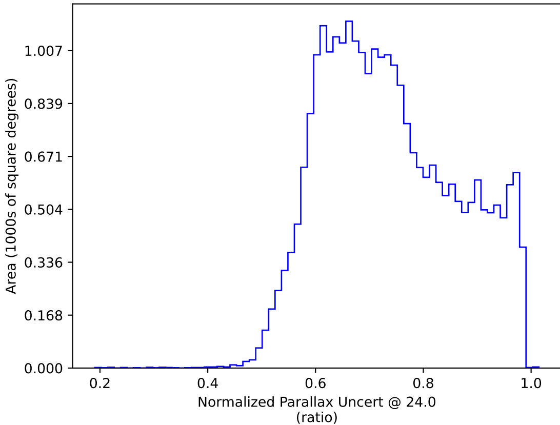
too_elab_r8_d3_gz_v3.4_10yrs All sky: Normalized Parallax Uncert @ 24.0
