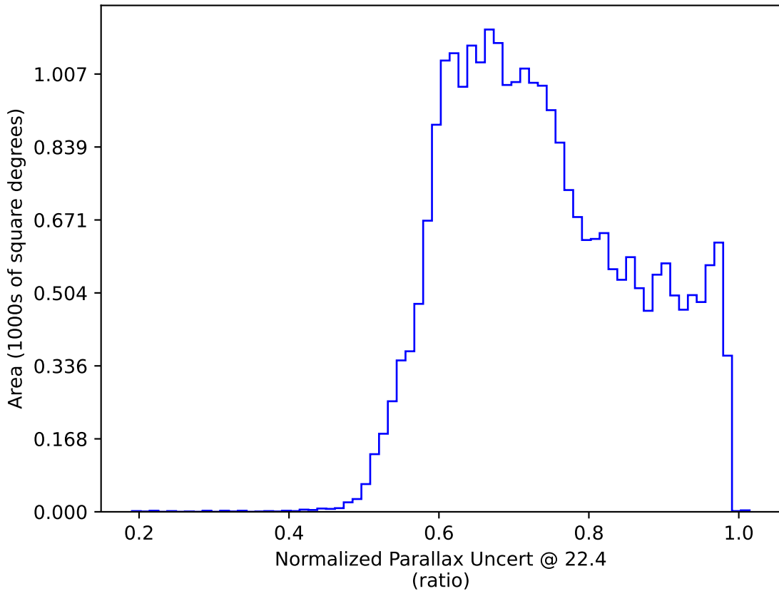
too_elab_r8_d3_gz_v3.4_10yrs All sky: Normalized Parallax Uncert @ 22.4
