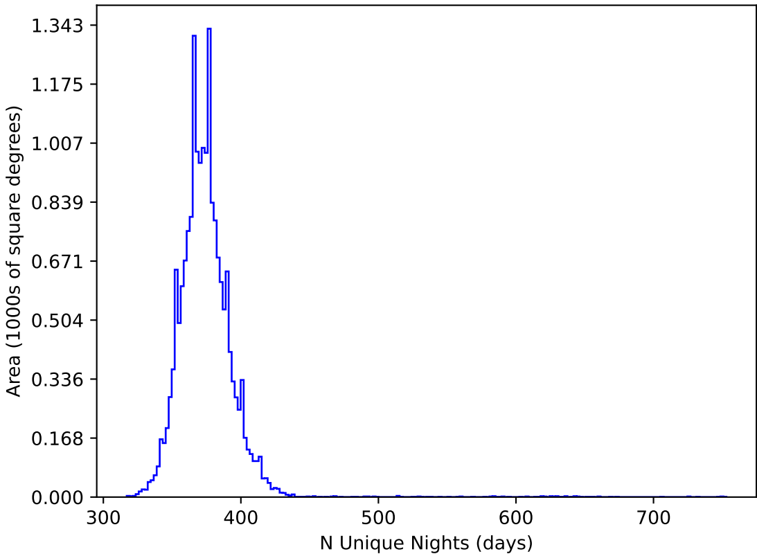
too_elab_r8_d3_gz_v3.4_10yrs WFD all bands: N Unique Nights
