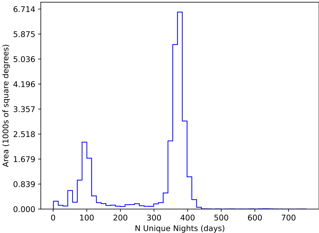
too_elab_r8_d3_gz_v3.4_10yrs All sky all bands: N Unique Nights
