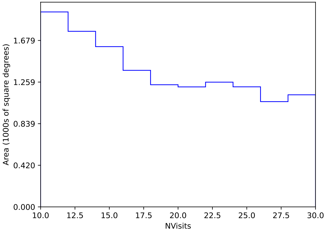
too_elab_r8_d3_gz_v3.4_10yrs Yr 3-4 y band: NVisits
