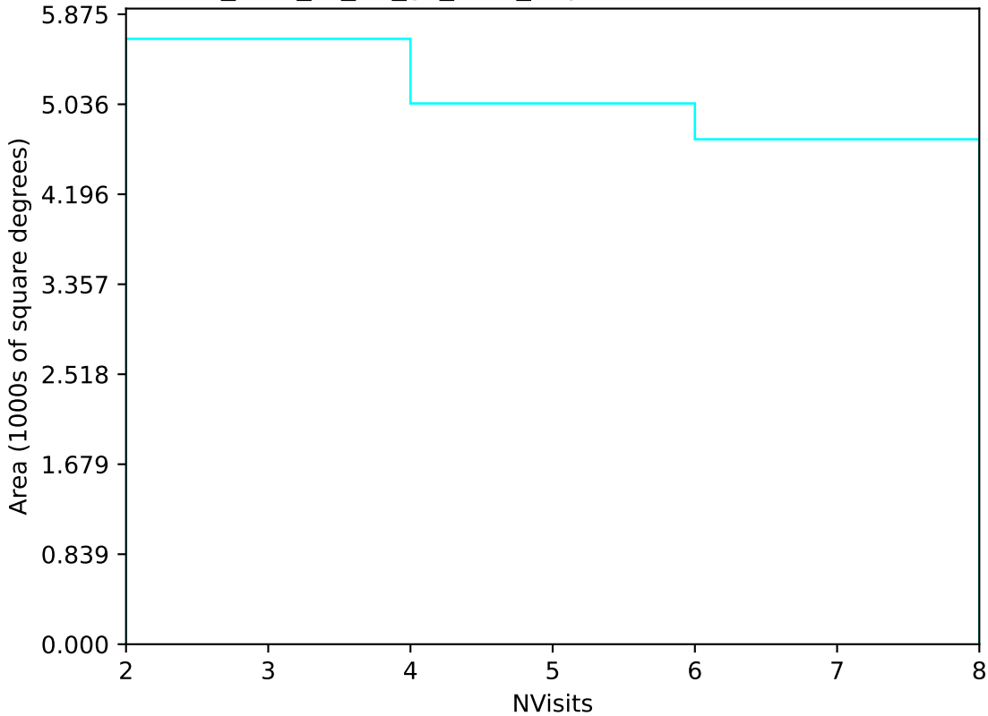
too_elab_r8_d3_gz_v3.4_10yrs Yr 3-4 u band: NVisits
