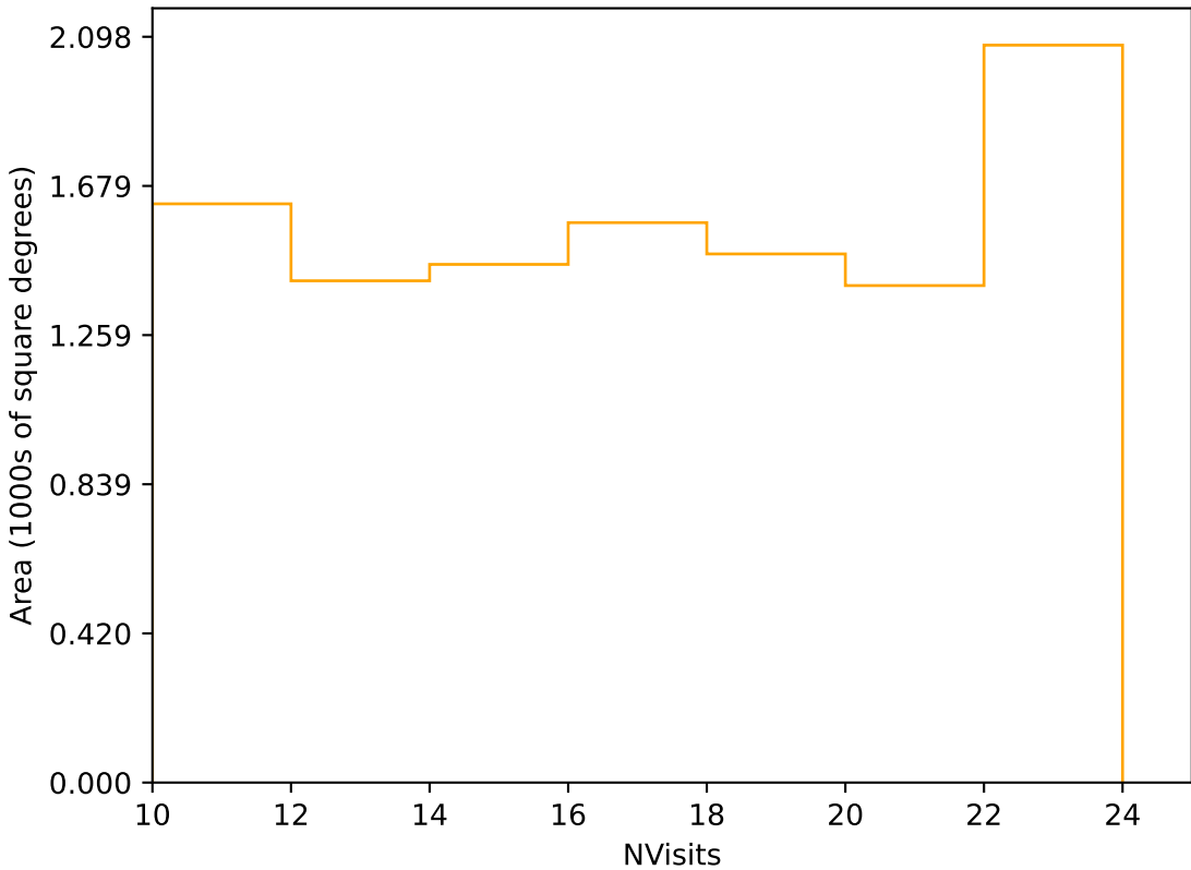
too_elab_r8_d3_gz_v3.4_10yrs Yr 3-4 r band: NVisits
