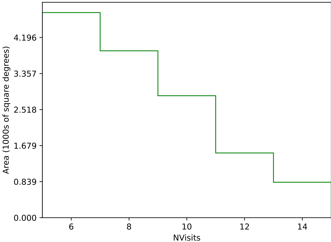
too_elab_r8_d3_gz_v3.4_10yrs Yr 3-4 g band: NVisits
