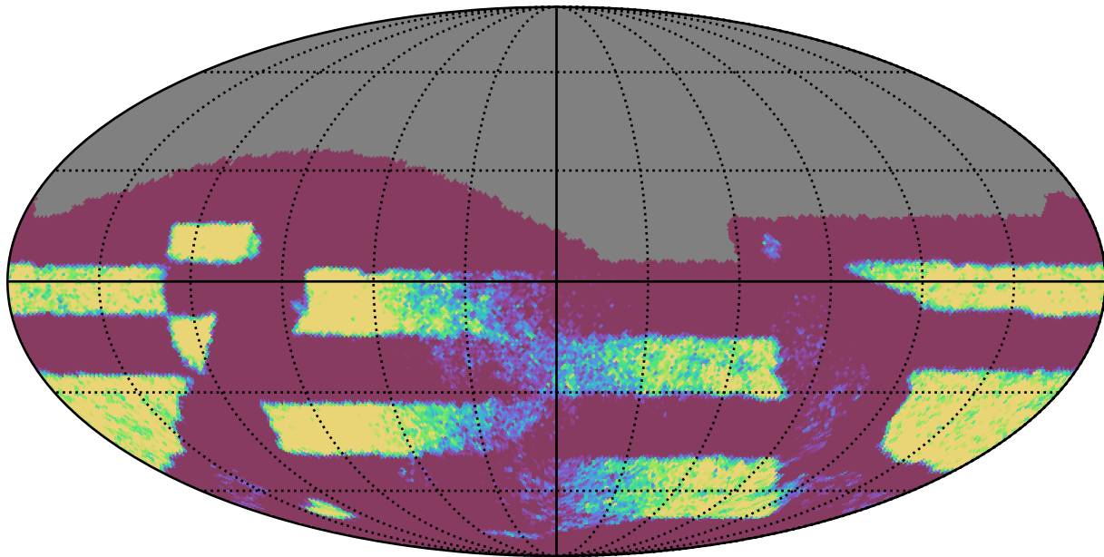
too_elab_r8_d3_gz_v3.4_10yrs Yr 3-4 all bands: NVisits
