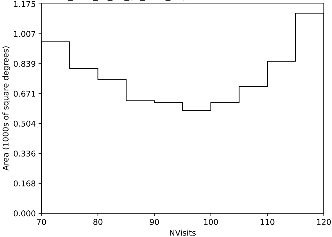
too_elab_r8_d3_gz_v3.4_10yrs Yr 3-4 all bands: NVisits
