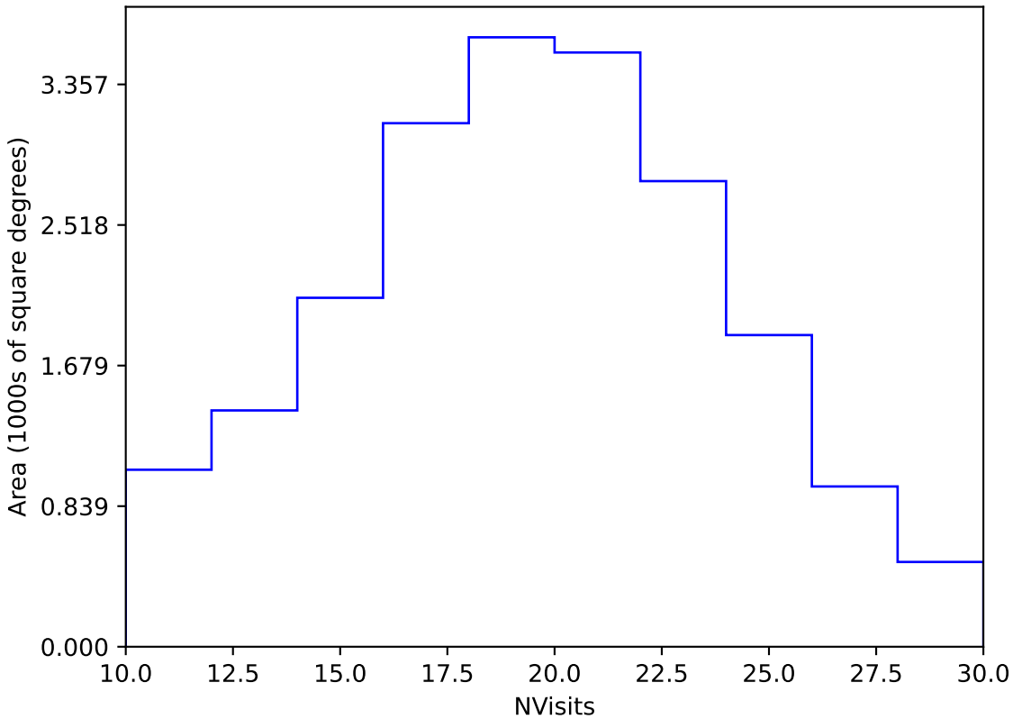
too_elab_r8_d3_gz_v3.4_10yrs Yr 1 y band: NVisits
