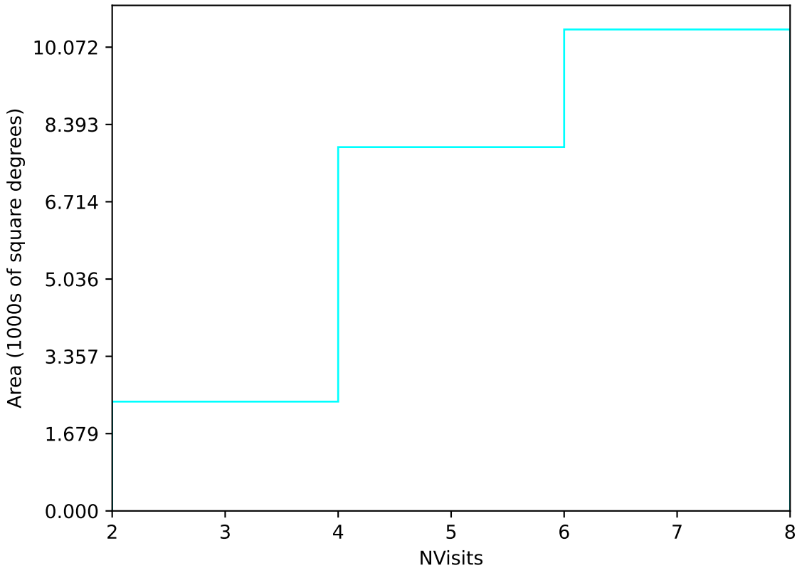
too_elab_r8_d3_gz_v3.4_10yrs Yr 1 u band: NVisits
