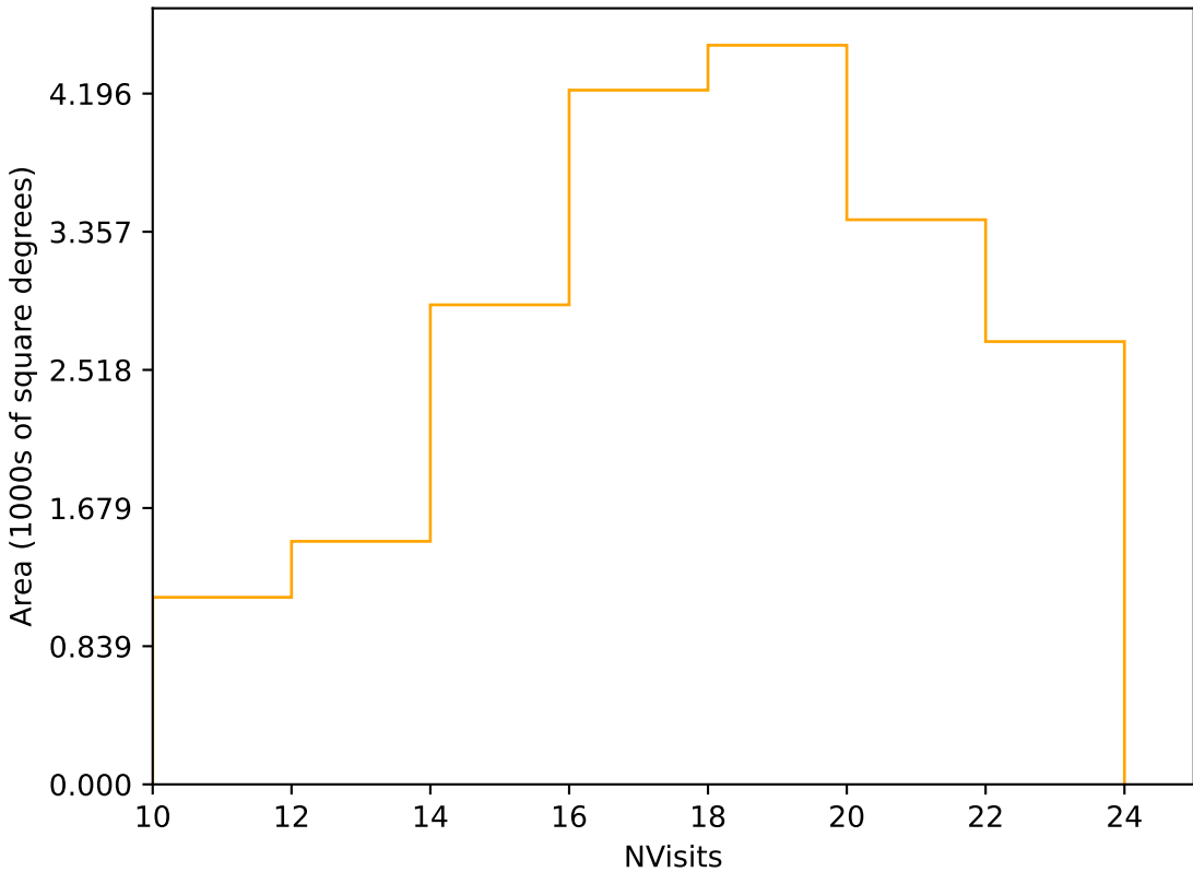
too_elab_r8_d3_gz_v3.4_10yrs Yr 1 r band: NVisits
