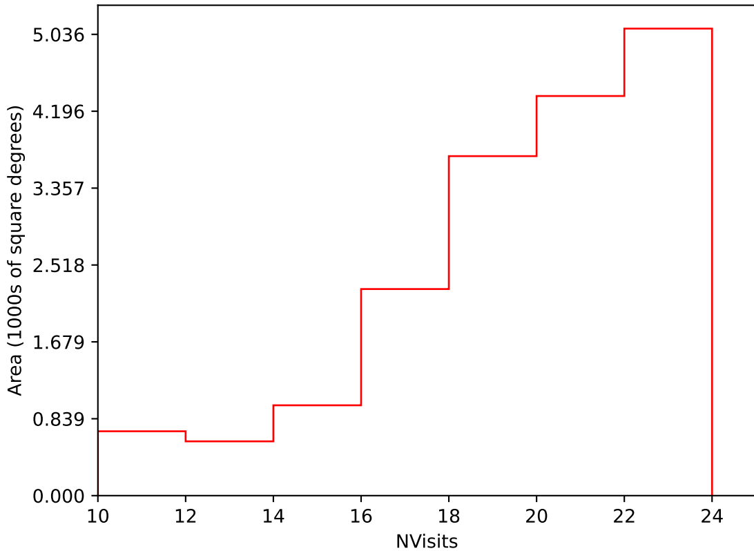
too_elab_r8_d3_gz_v3.4_10yrs Yr 1 i band: NVisits
