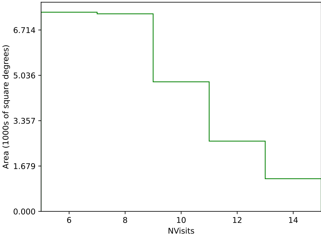
too_elab_r8_d3_gz_v3.4_10yrs Yr 1 g band: NVisits
