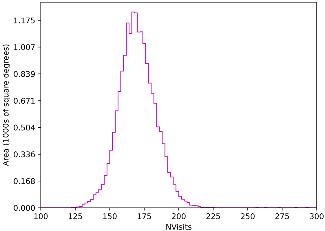
too_elab_r8_d3_gz_v3.4_10yrs WFD z band: NVisits
